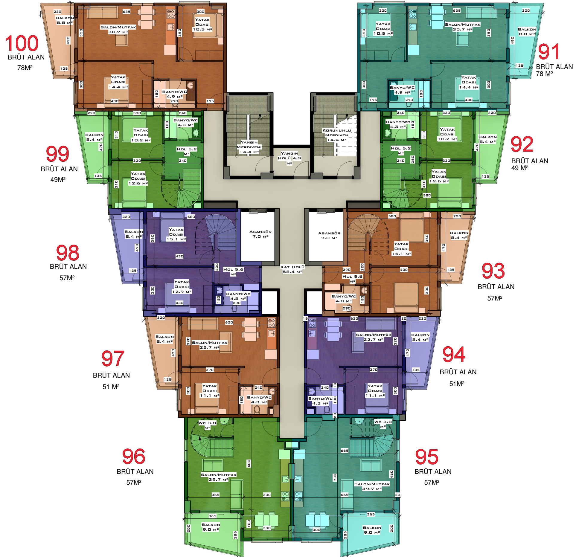
DUBLEKS ALT KAT PLANI
