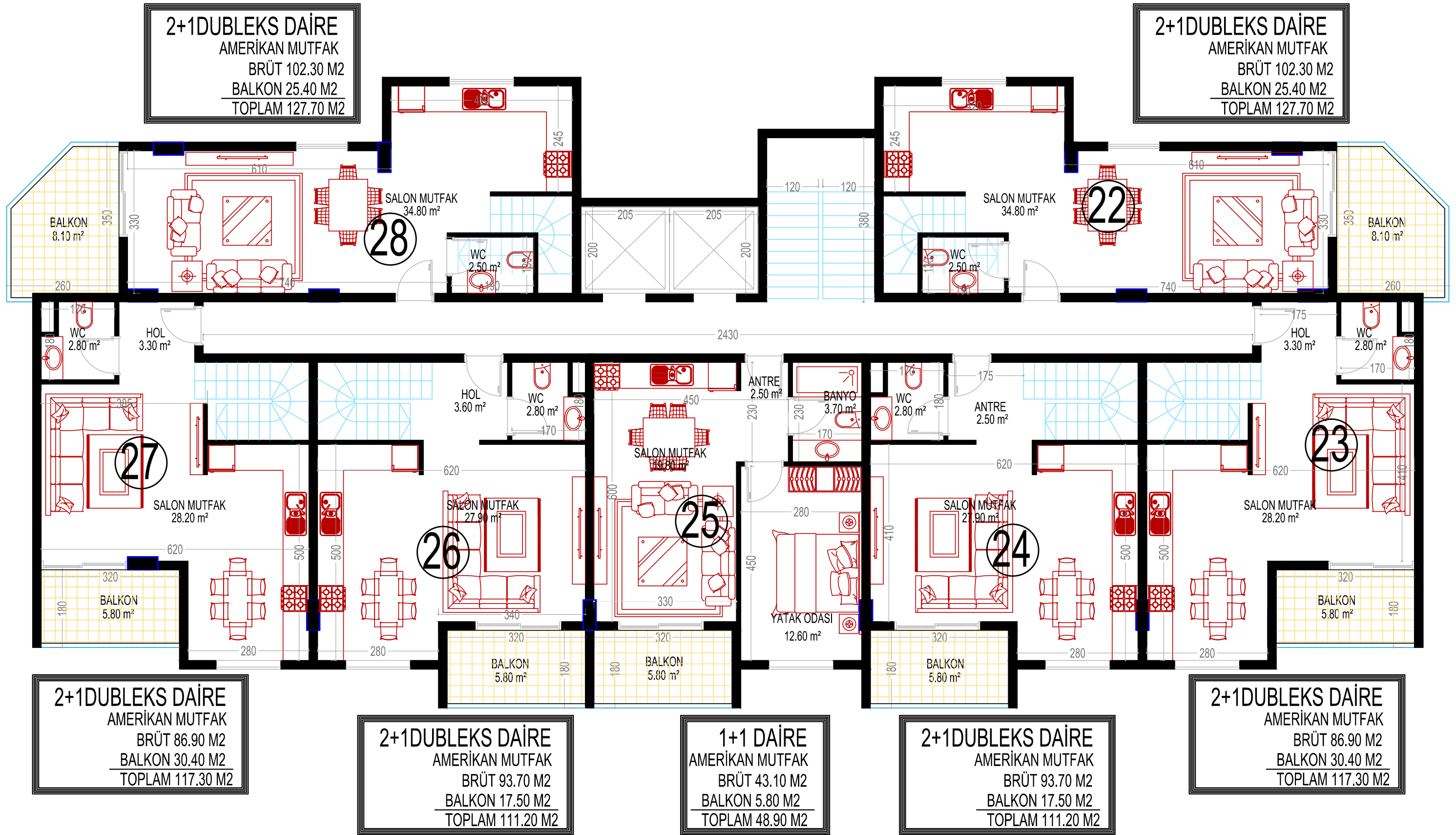
DUBLEKS 1. KAT PLANI
